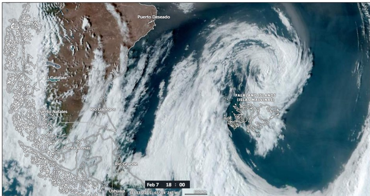
Figure 5. Image of the Dragonhead cyclone, at 6 pm (UTC), February 7, 2024. Source: [57, Adapted Authors]
